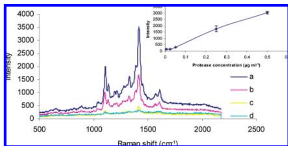
Figure 3. SERRS obtained from 4 upon exposure to Subtilisin carlsberg, at concentration of (a) 0.5 , (b) 0.25 , (c) 0.05 , and (d) 0.005 \text{ } \mu\text{g ml}^{-1} . (Inset) Enzyme concentration against SERRS response at 1419 \text{ cm}^{-1} . Reaction time is 30 min.
