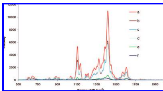
Figure 2. SERRS obtained from 4 upon 30 min treatment with (a) \alpha -Chymotrypsin, (b) Subtilisin carlsberg, (c) Trypsin, (d) Proteinase K, (e) Pepsin, (f) blank, in each case with the enzyme concentration at 0.01 \text{ mg ml}^{-1} .
